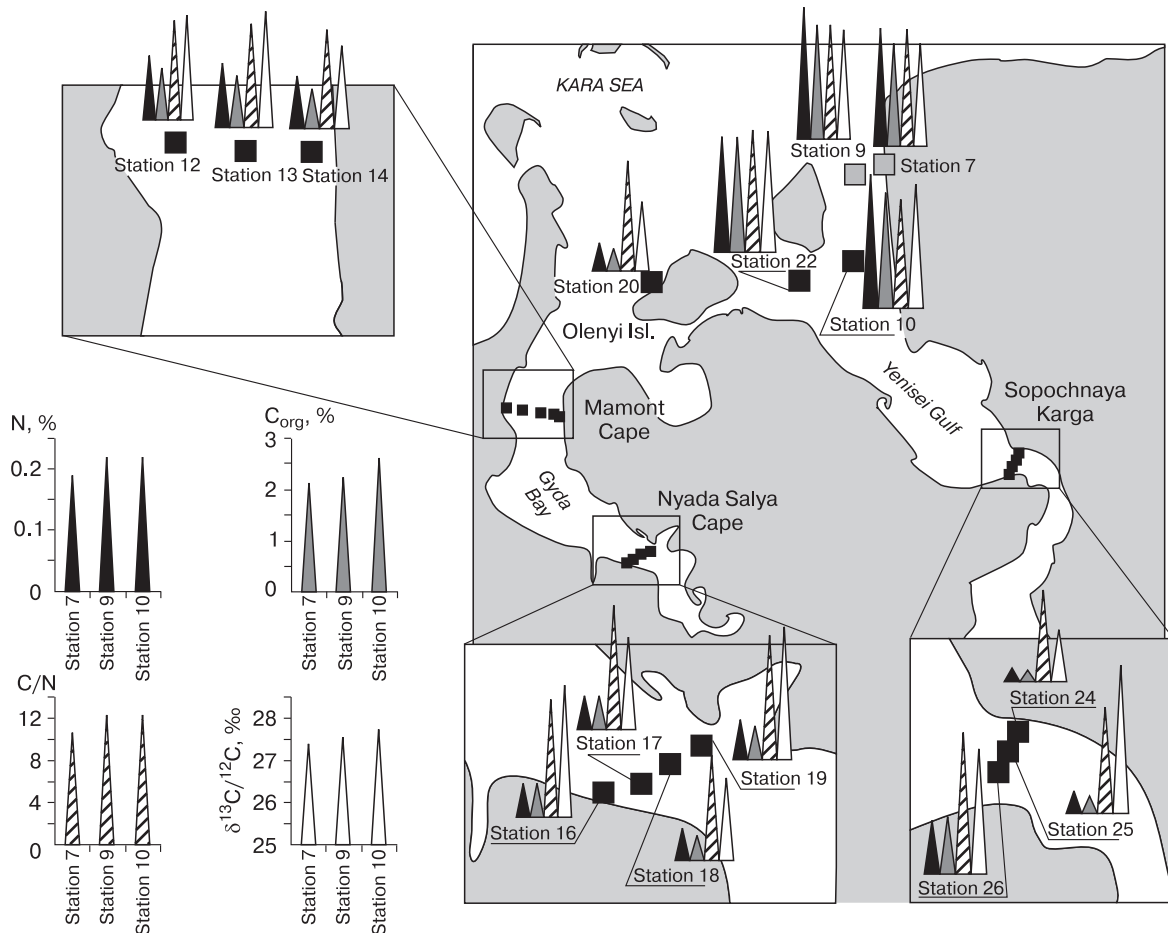
Fig. 1. Location map of sampling sites in lower Yenisei, Gyda Bay, and Kara shelf, with contents of organic nitrogen ( N_{org} ) and organic carbon ( C_{org} ), C_{org}/N_{org} ratios, and carbon isotope composition ( \delta^{13}C/^{12}C ) in surface bottom sediments.
